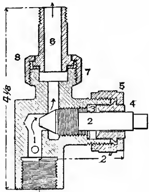
Fig. 3116. Section. CLOSET-VALVE.
